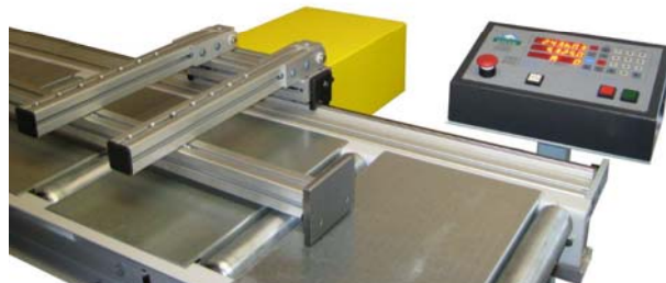
PD50 stop arm in lift position
