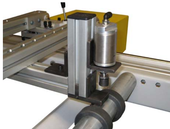
PD50 pneumatic gripper (vertical with pass thru collars)
